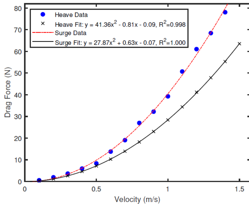
Fig. 4. Drag Force as a Function of Velocity in different Directions
